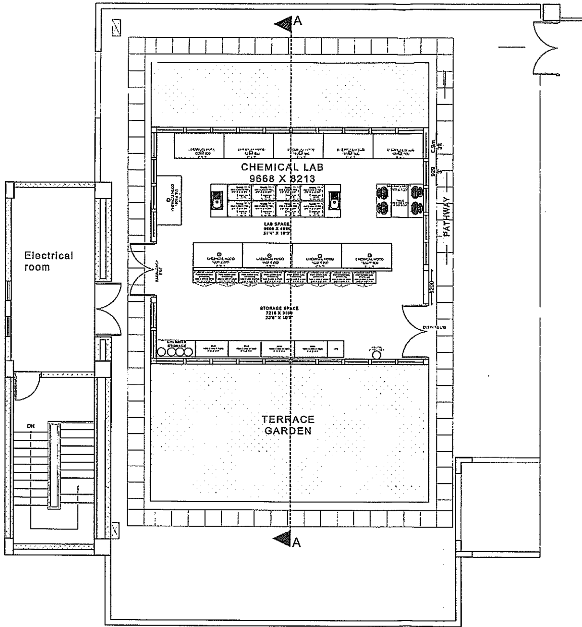
PLAN
