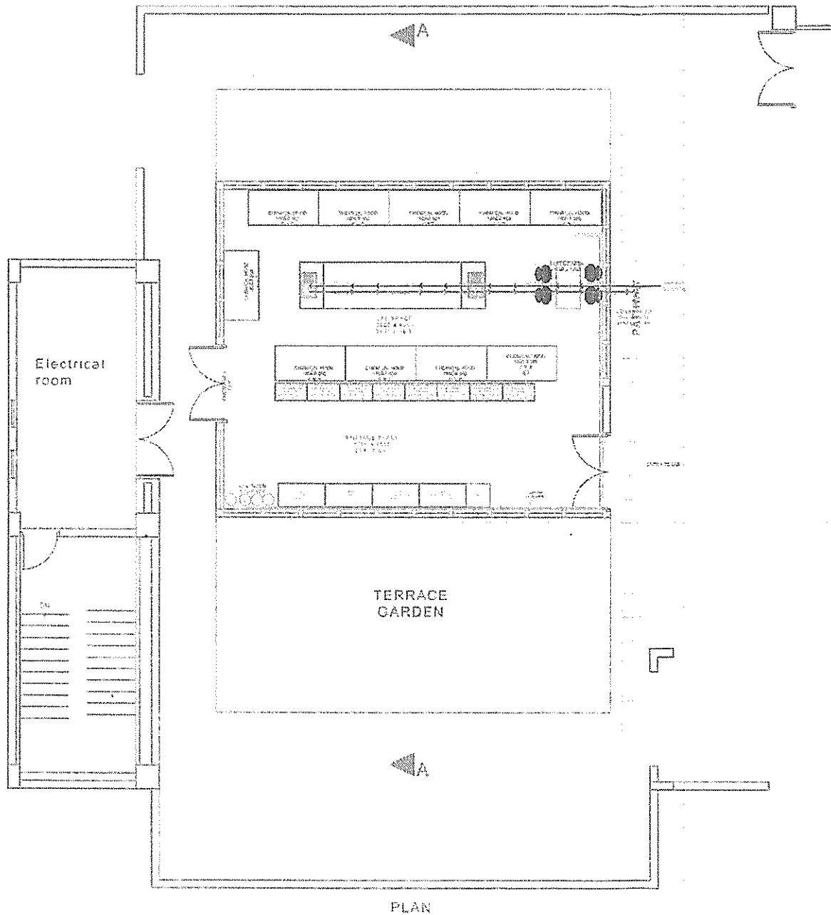
PLAN
